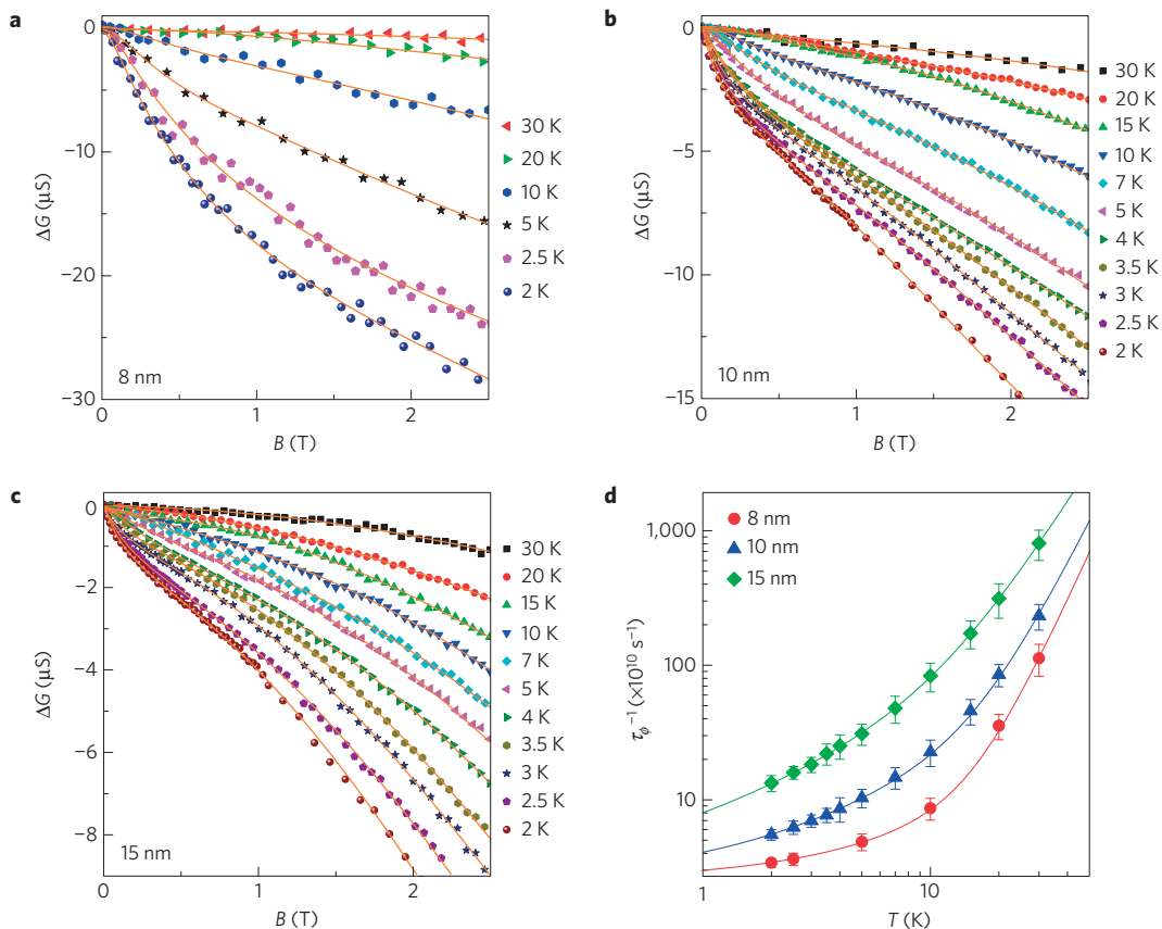
Figure 4 | Thickness and temperature dependences of electron phase coherence in \text{Nb}_3\text{SiTe}_6 thin crystals. a–c , Fits of the magnetotransport data up to B = 2.5 T for 8 nm ( a ), 10 nm ( b ) and 15 nm ( c ) \text{Nb}_3\text{SiTe}_6 thin-flake crystals to the 2D WAL model (HLN model). d , Temperature dependence of the dephasing rate \tau_{\phi}^{-1} for the 8, 10 and 15 nm samples, obtained from the fittings shown in a–c . Error bars represent uncertainties in the fits. The solid lines show the fits for the temperature dependence of \tau_{\phi}^{-1} (see text).
