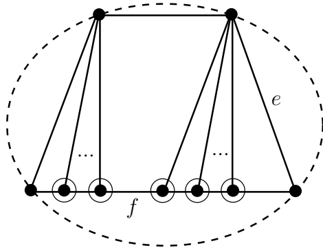
Figure 3.40. Adding e to create a (k + 1) -fan.
