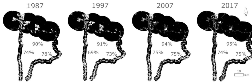
FIGURE 3 Results of land cover classification as closed-canopy forest (primary forest or mature regrowth; black) and nonforest (white) using Landsat imagery across 30 years at the Biological Dynamics of Forest Fragments Project (BDFFP) and along two highways that connect the city of Manaus, Brazil, to the BDFFP. The percent of forest within the BDFFP and along each of the two corridors (BR-174 to the west and AM-010/ZF-7 to the east) is illustrated during all four time periods
